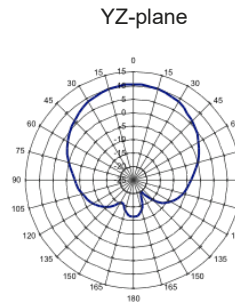
Portal antennas (two sides & top)
